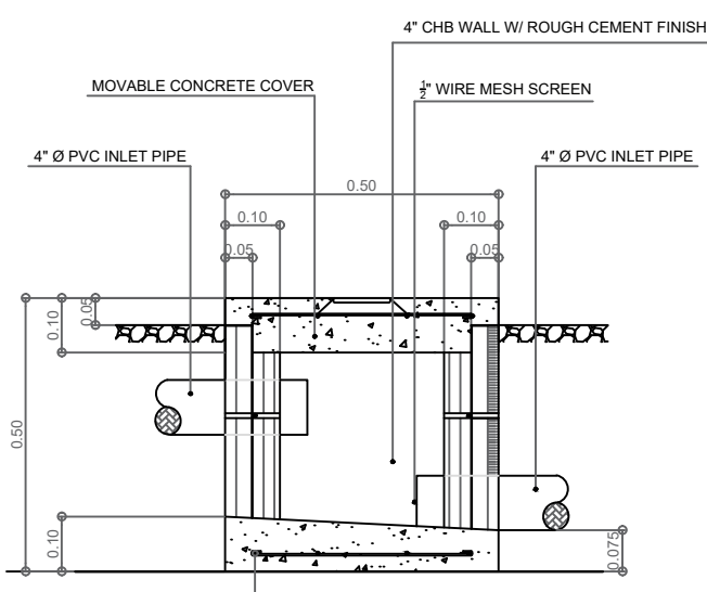
5 CATCH BASIN DETAILS P1 P1 SCALE 1 : 15 M.
