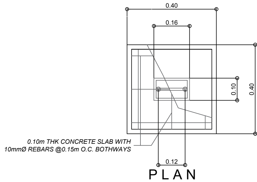
4 MANHOLE DETAILS P1 P1 SCALE 1 : 10 M.
