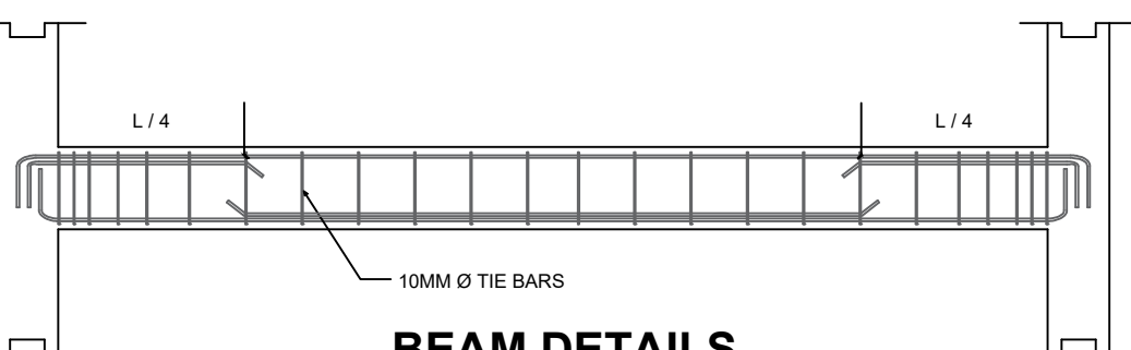
BEAM DETAILS
