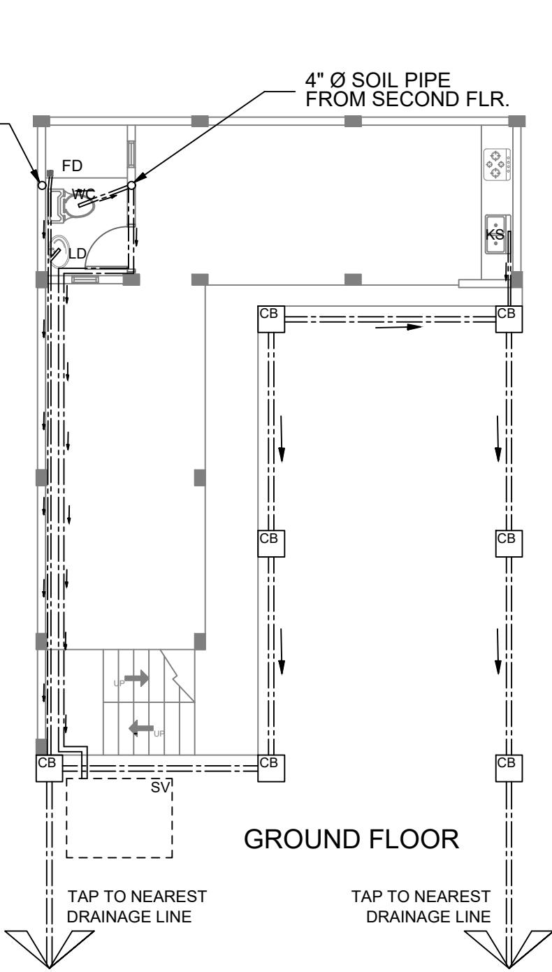
2 SANITARY LAYOUT P1 P1 SCALE 1 : 100 M.
