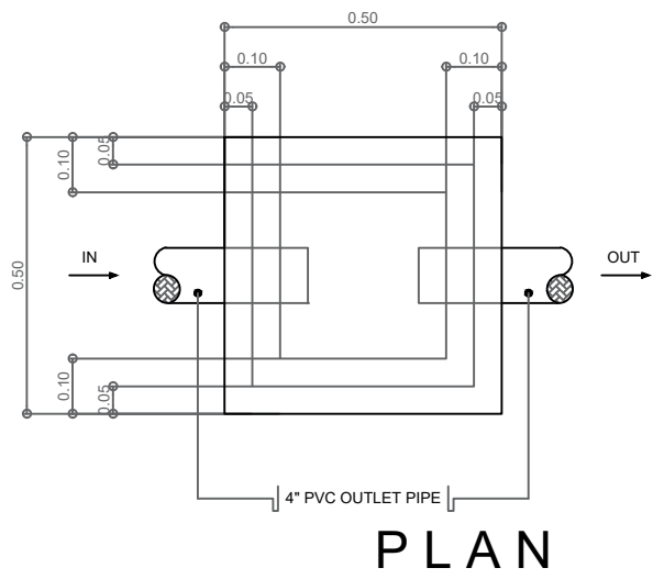
5 CATCH BASIN DETAILS P1 P1 SCALE 1 : 15 M.
