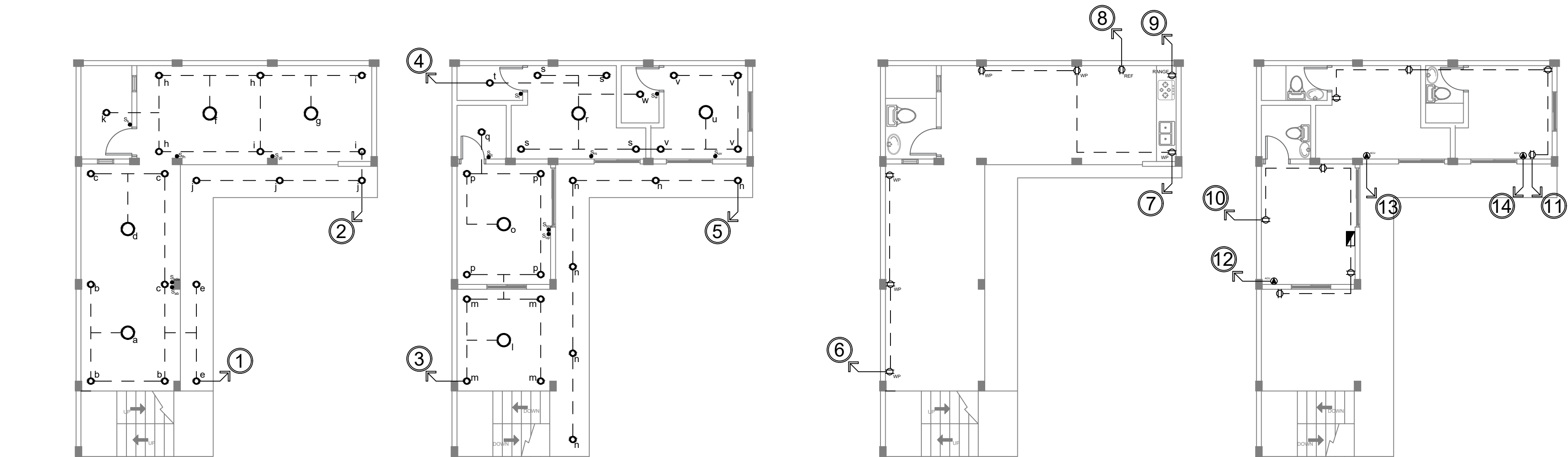
GROUND FLOOR SECOND FLOOR 1 LIGHTING LAYOUT SCALE 1 : 100 M.
