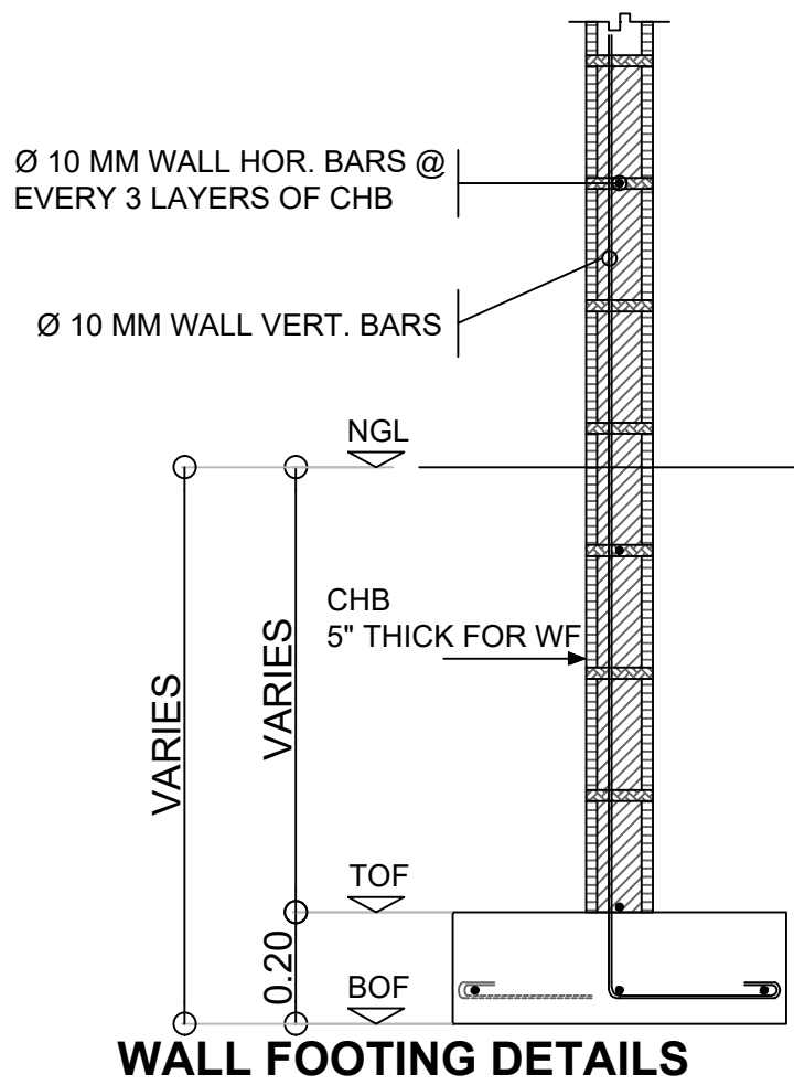
WALL FOOTING DETAILS
