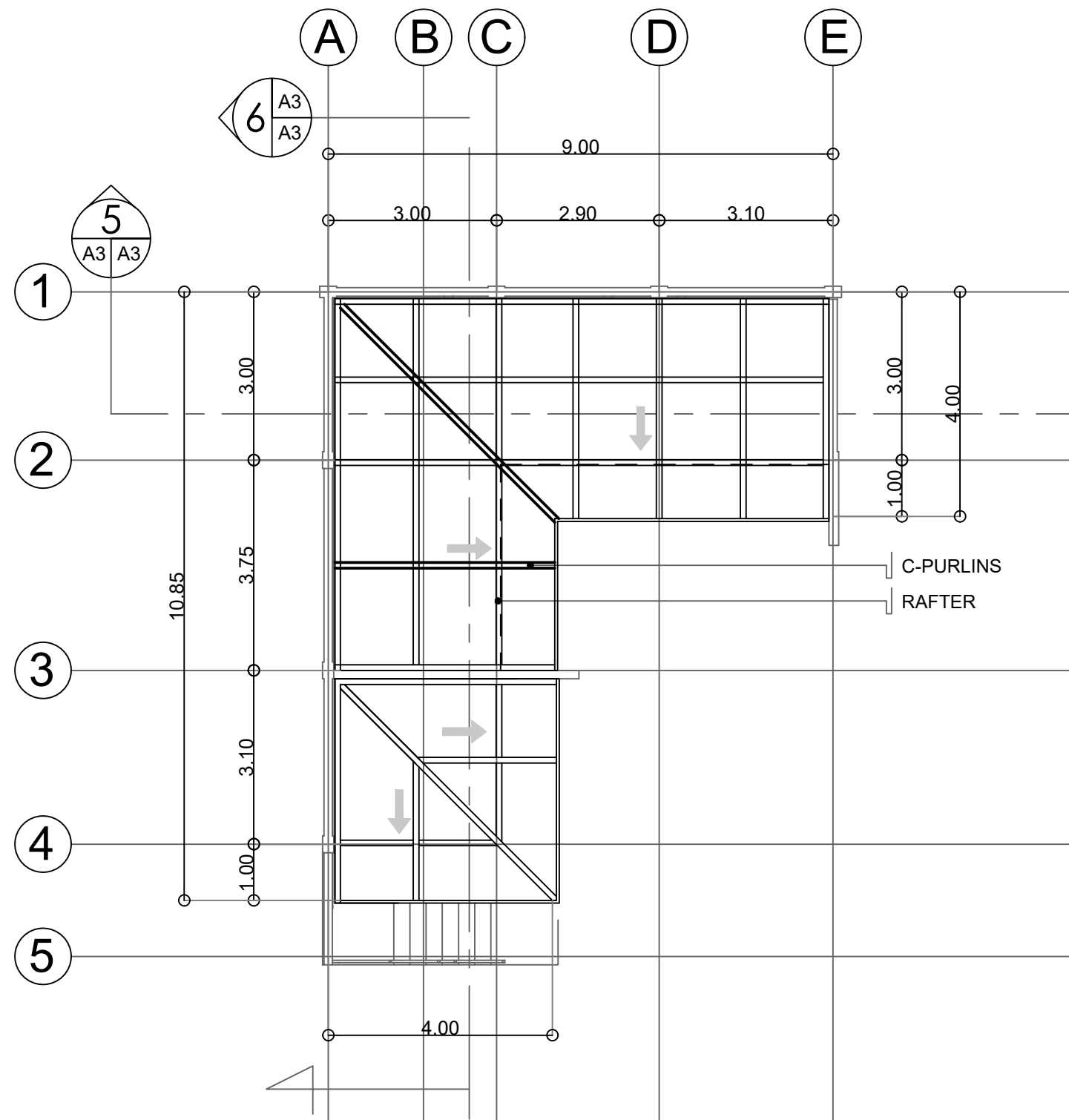
1 ROOF FRAMING PLAN S2 S2 SCALE 1 : 100 M.
