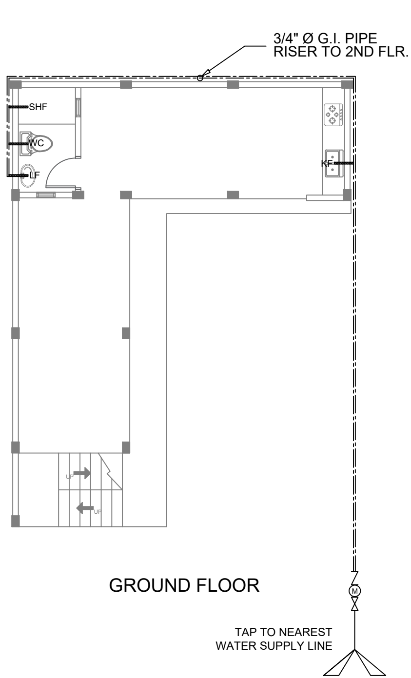
1 WATER DISTRIBUTION LAYOUT P1 P1 SCALE 1 : 100 M.
